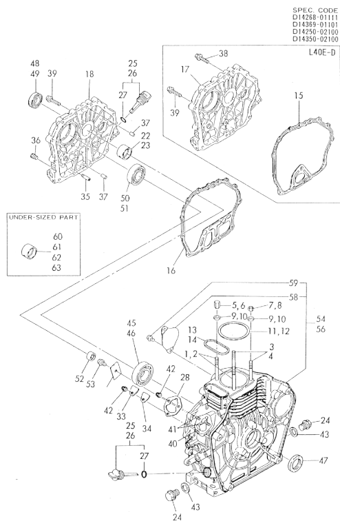
Fig.1. CYLINDER BLOCK
