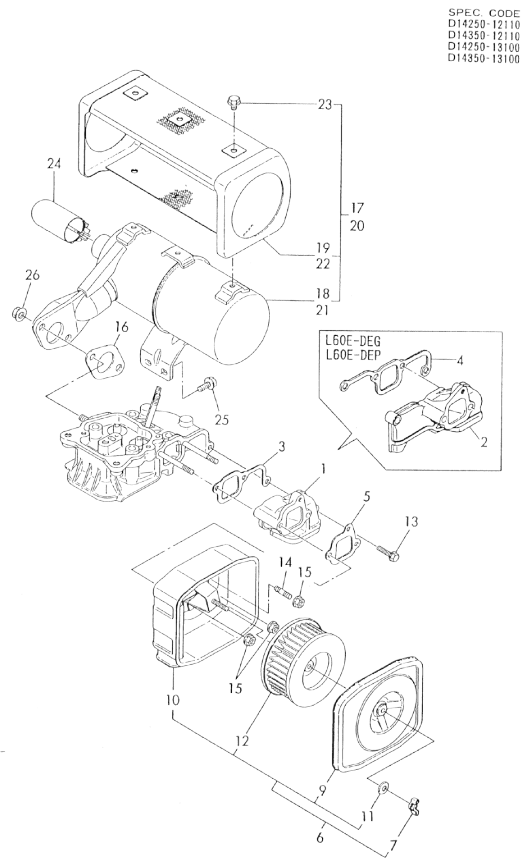
Fig.3. AIR CLEANER & MUFFLER
