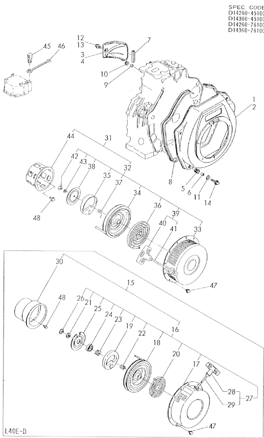
Fig.6. COOLING & STARTING DEVICE
