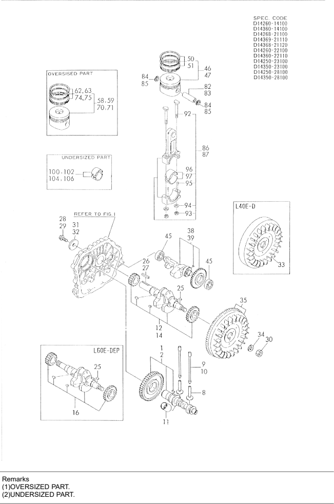
Fig.4. CRANKSHAFT,PISTON & CAMSHAFT
