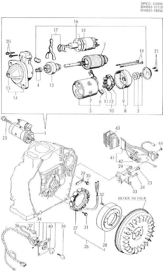
Fig.9. STARTING MOTOR & DYNAMO
