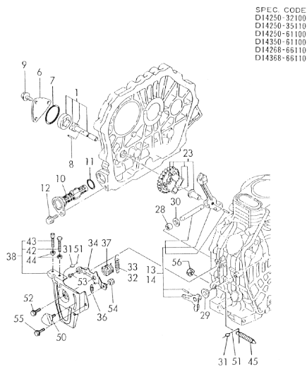
Fig.5. LUB. OIL PUMP & GOVERNOR
