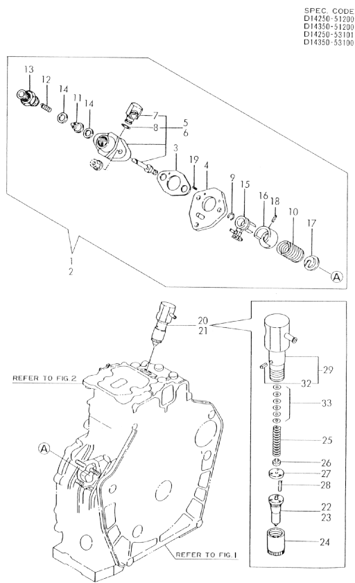
Fig.7. FUEL INJECTION PUMP
